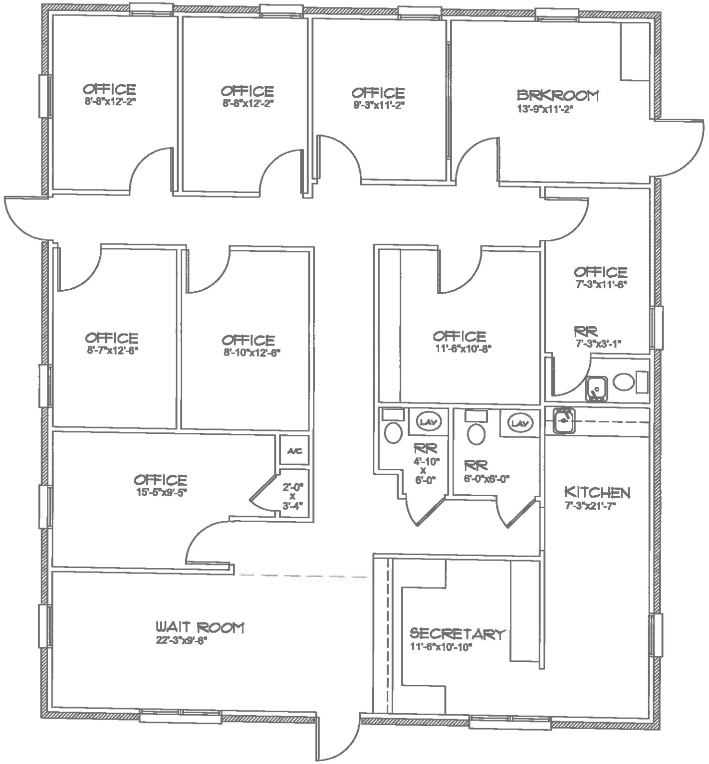
LEASE SPACE 1403 BUILDING G 2135 SQ. FT.
